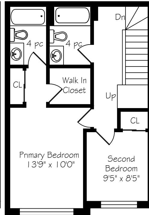
Third Floor 552 Square Feet
